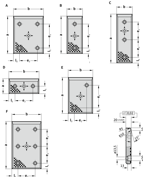
2211. Self-lubricating guide plate, ISO 9183-1
